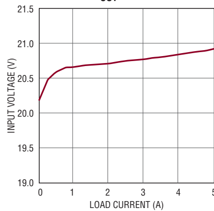
Minimum Required Input Voltage vs Load 18V OUT
