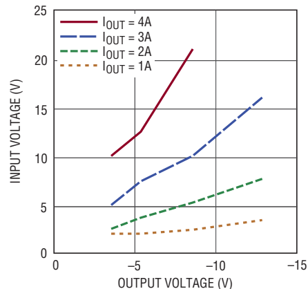
Minimum Required Input Running Voltage vs Negative Output Voltage
